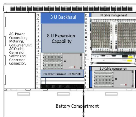
Figure 2: Example Cabinet Configuration
